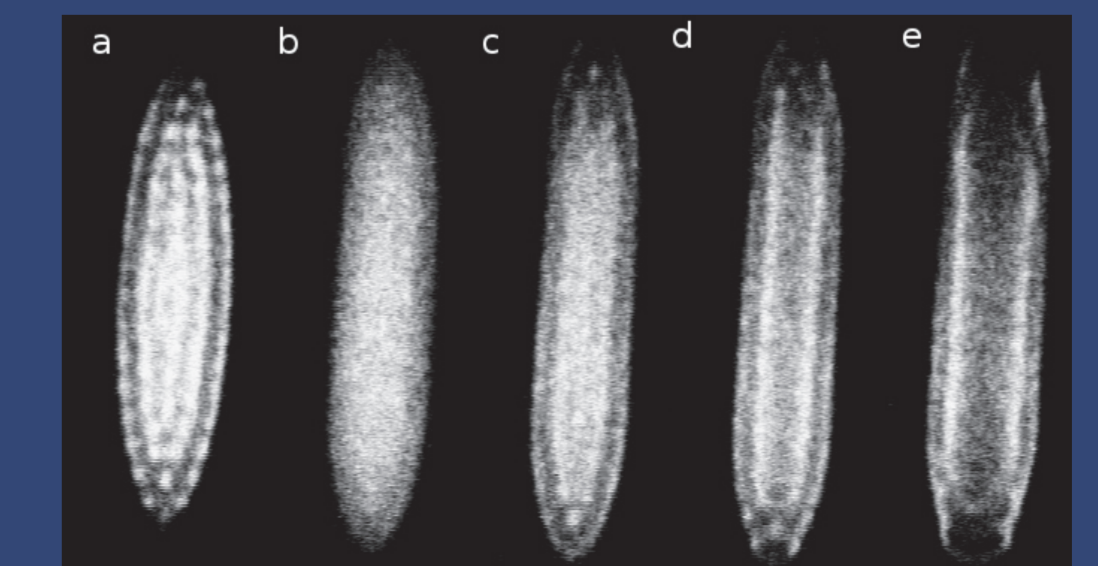
Coulomb crystal Xe^+ + NH_3 reaction sequence
