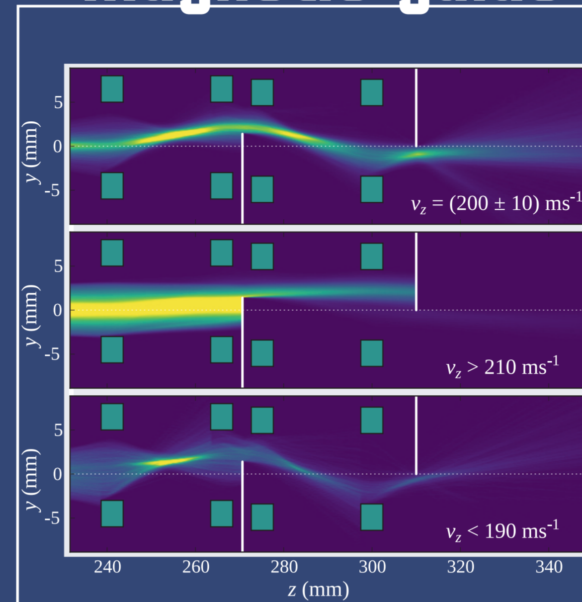
Magnetic velocity Filter
