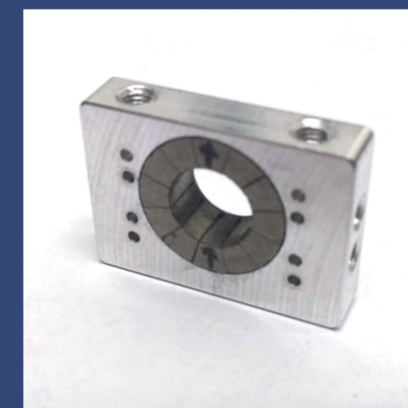
Building element Halbach array
