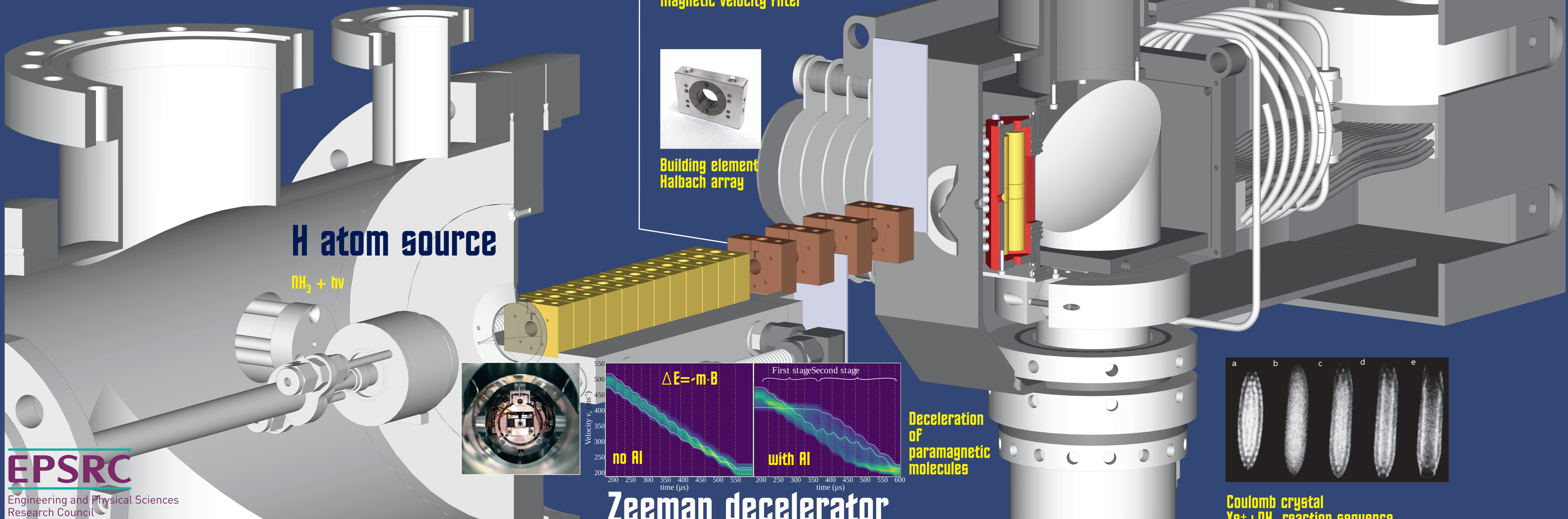
Magnetic velocity Filter
